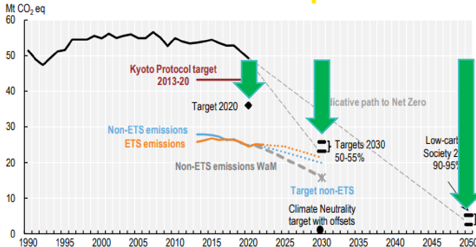
Norway's historical and projected GHG emissions (without LULUCF)
